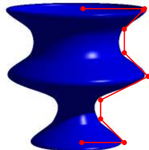
Cubic Spline
