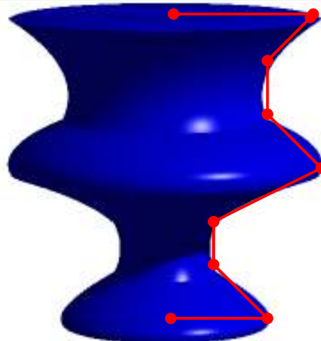
Quadratic Spline
