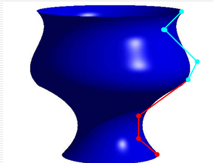
Bezier Spline
